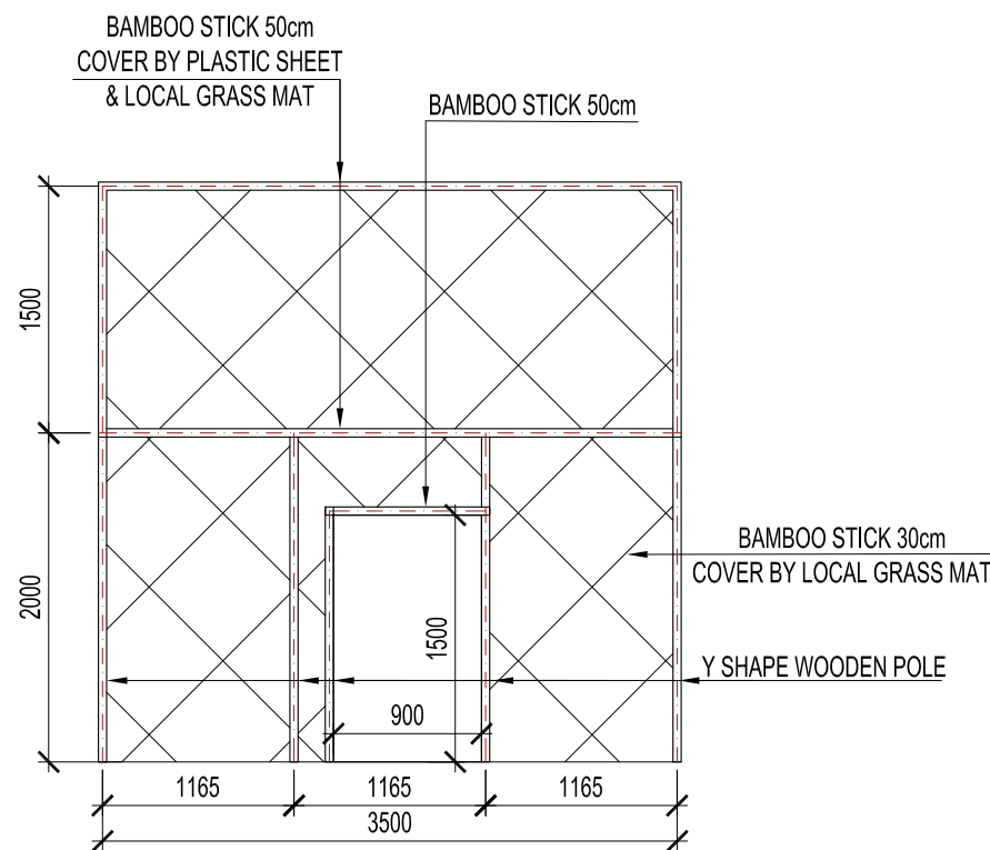
ELEVATION 01 SCALE (1:50)
