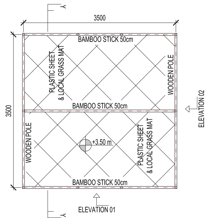
ROOF LAYOUT SCALE (1:50)
