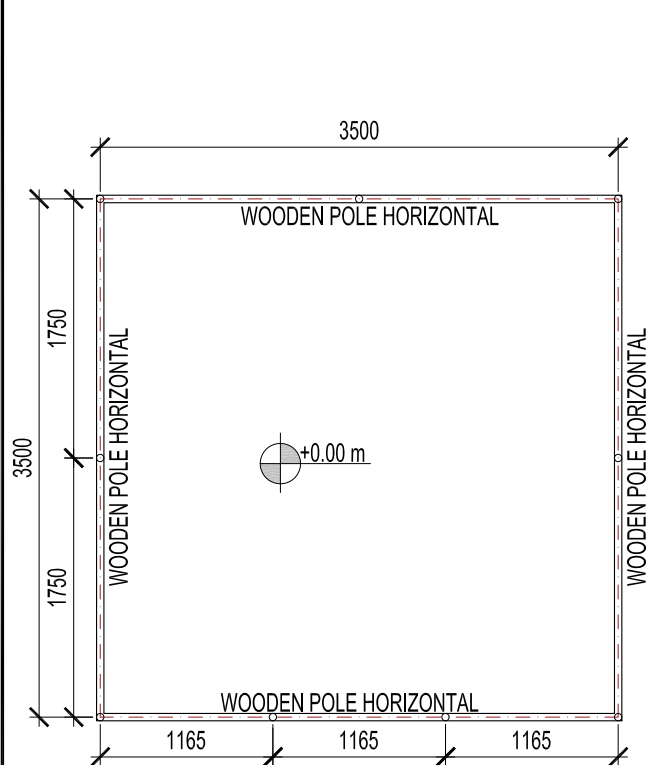
POLES LAYOUT SCALE (1:50)
