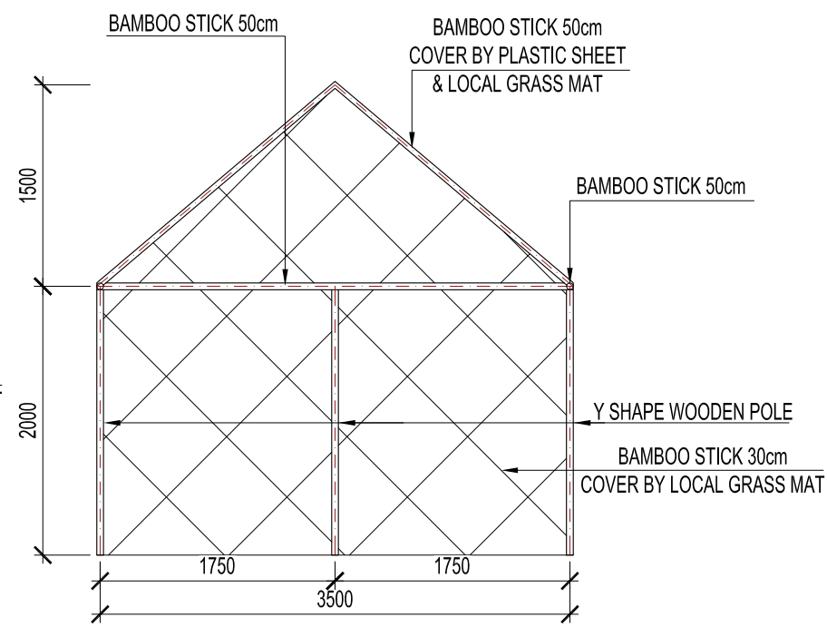
ELEVATION 02 SCALE (1:50)
