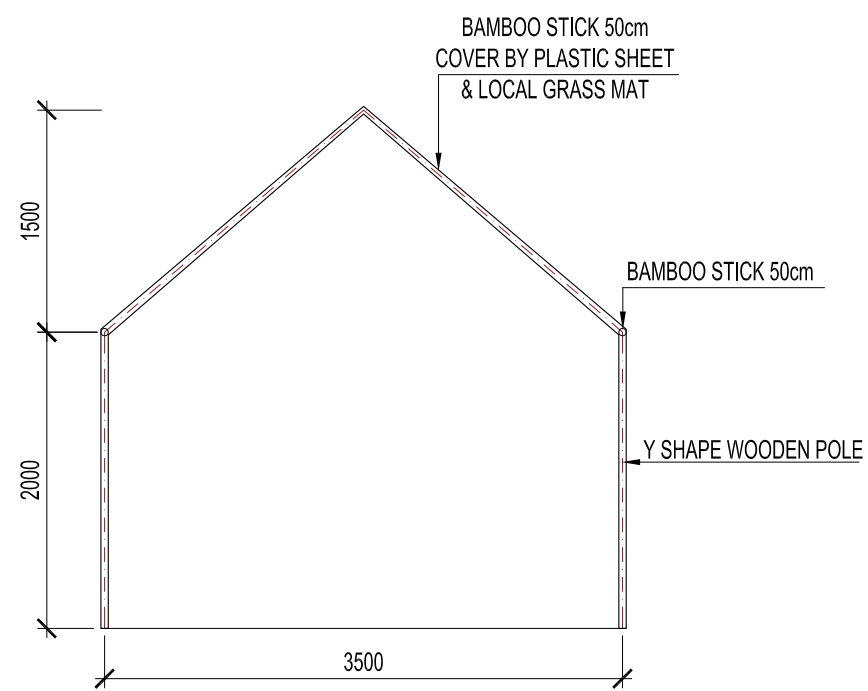
SECTION(Y-Y) SCALE (1:50)
