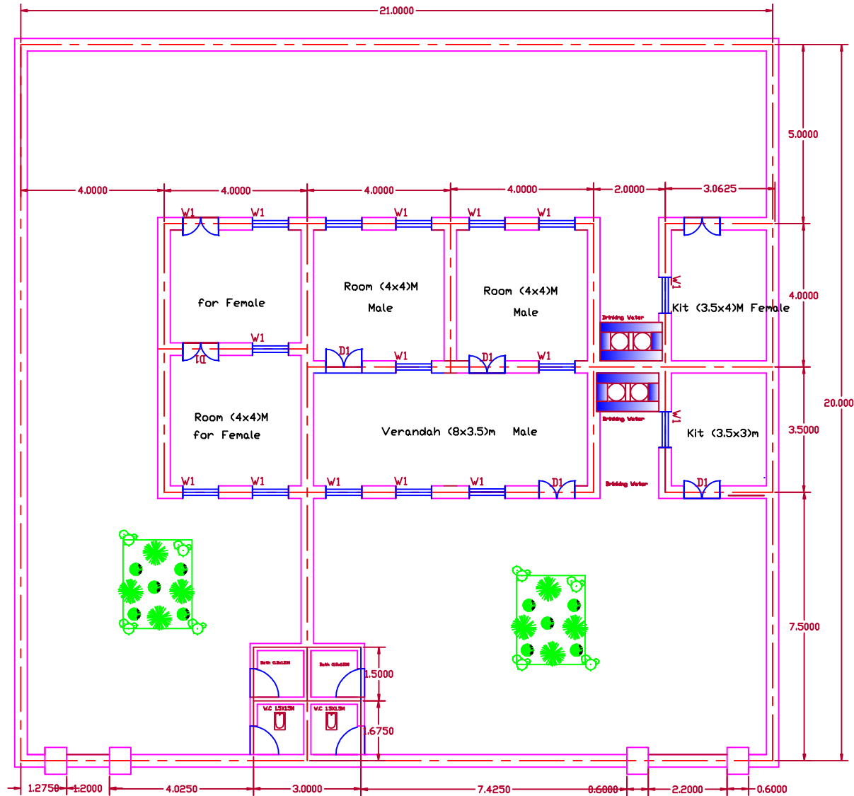
Teachers Accommodation for Male and female option 2 size (21x20)m
