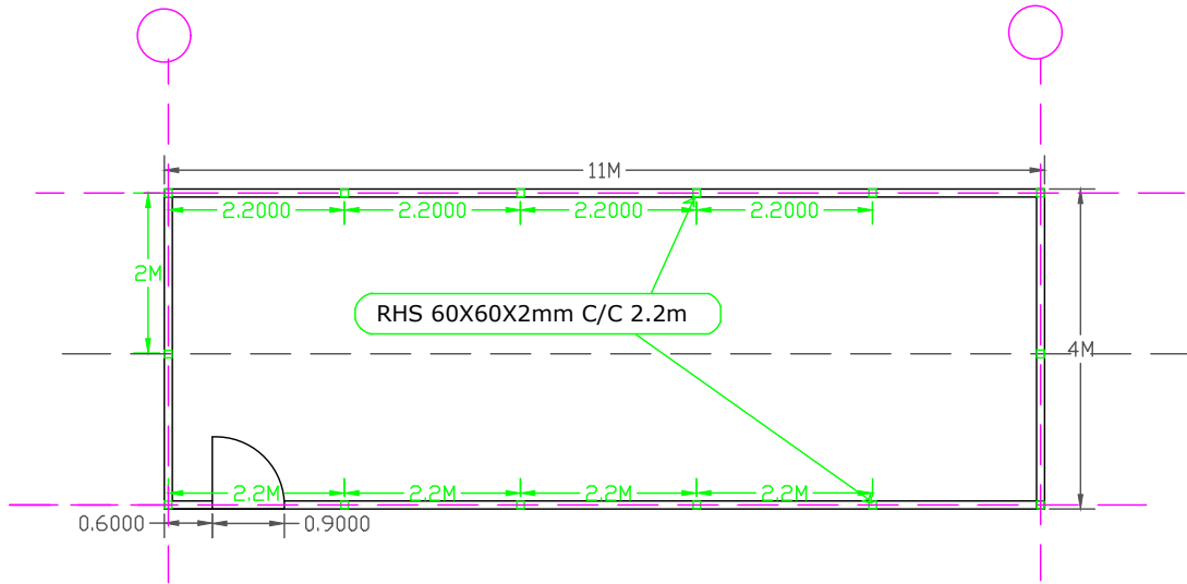
FLOOR PLAN
